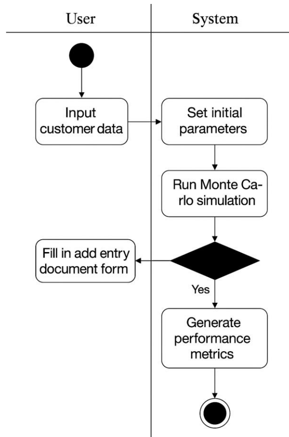
Figure 4. Activity Diagram
